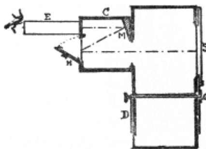
Vertical Section through light openings.
